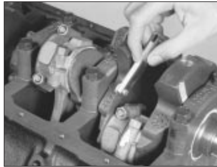
12.3 Check the connecting rod side play with a feeler gauge as shown
