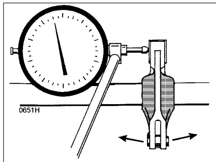
8.8 Check the rocker arm-to-shaft radial clearance by setting up a dial indicator as shown, and trying to rotate the rocker arm against the shaft - DO NOT slide the rocker arm along the shaft
