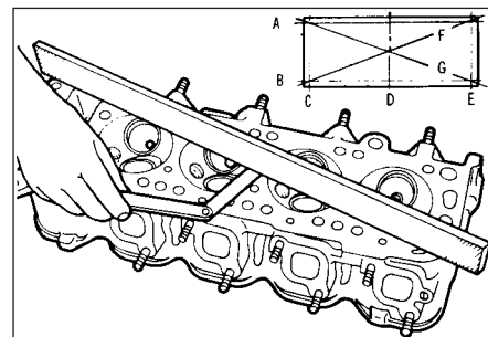
9.10 Check the cylinder head gasket surface for warpage by trying to slip a feeler gauge under the straightedge (see this Chapter's Specifications for the maximum warpage allowed, and use a feeler gauge of that thickness)
